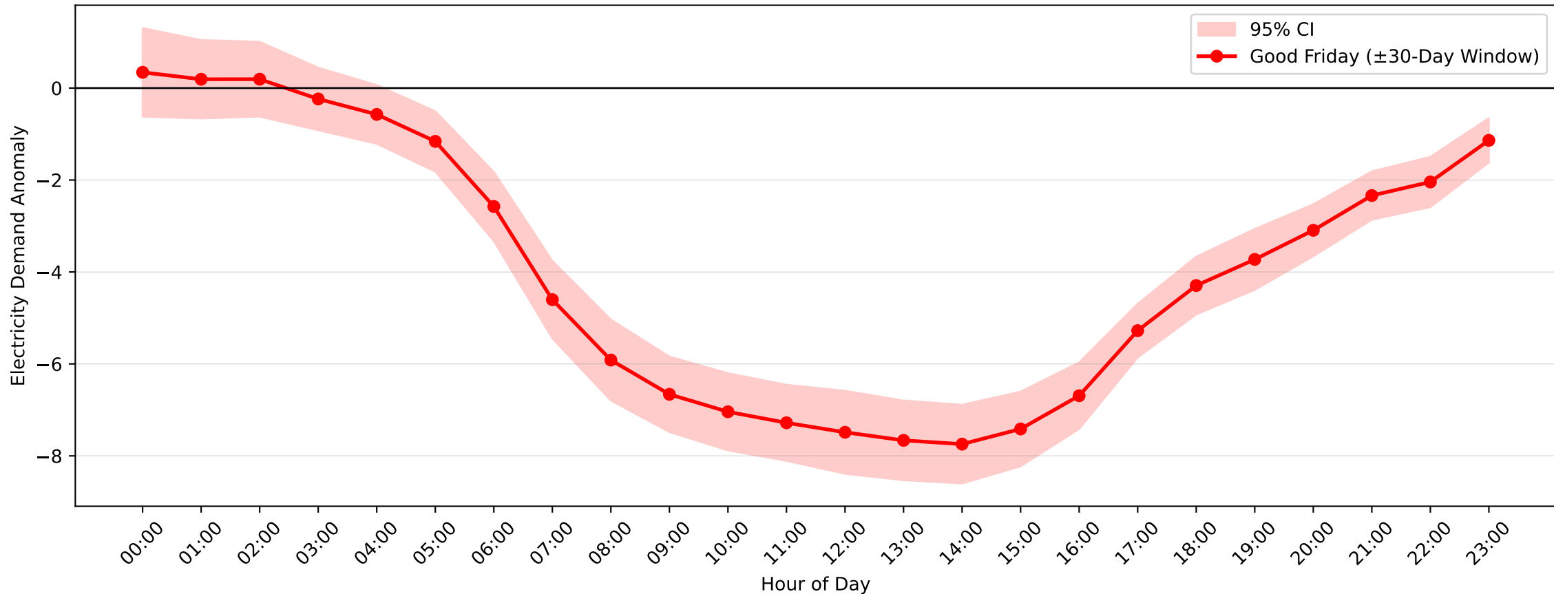
Newcastle Cbd Demand Anomaly: Good Friday (2004–2017, \pm 30 -Day Window)
